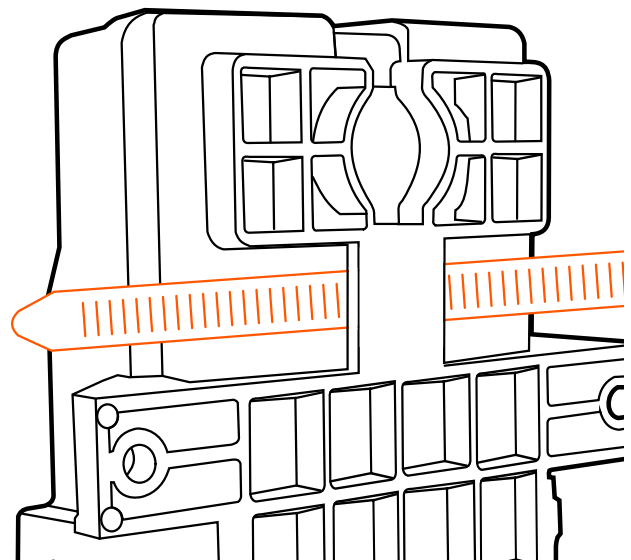
Figure 3. Mounting XO with a zip-tie.
