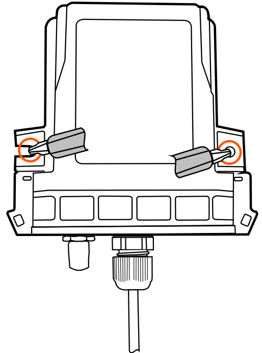
Figure 2. Mounting XO with screws.
